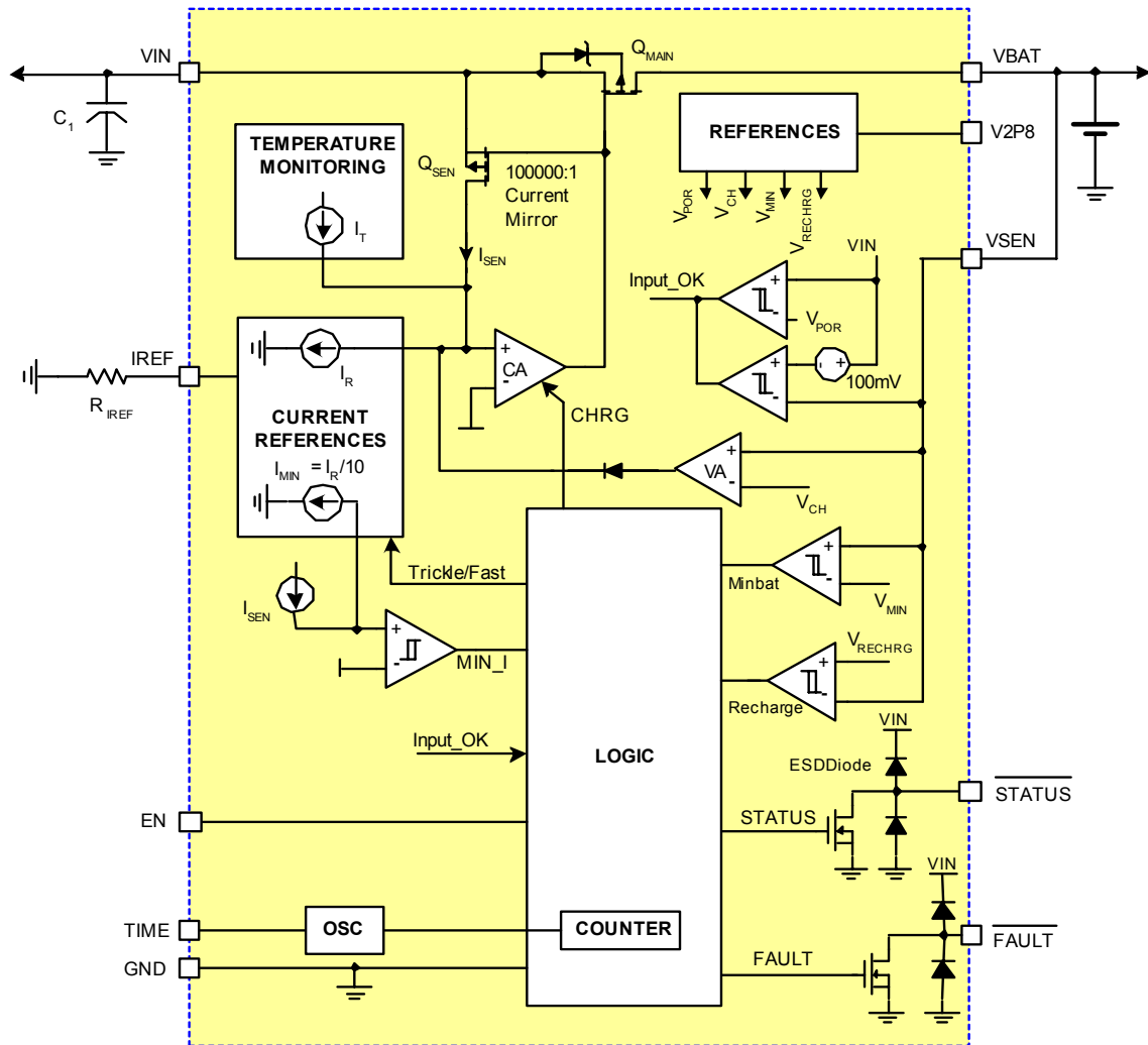
FIGURE 1. BLOCK DIAGRAM
