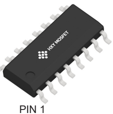
SOP-16 (SOIC-16)
