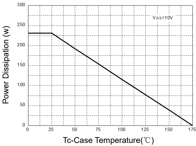
Figure 1: Power Dissipation
