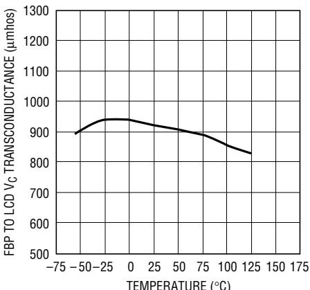
FBP to LCD V C Transconductance vs Temperature
