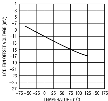
LCD FBN Offset Voltage vs Temperature
