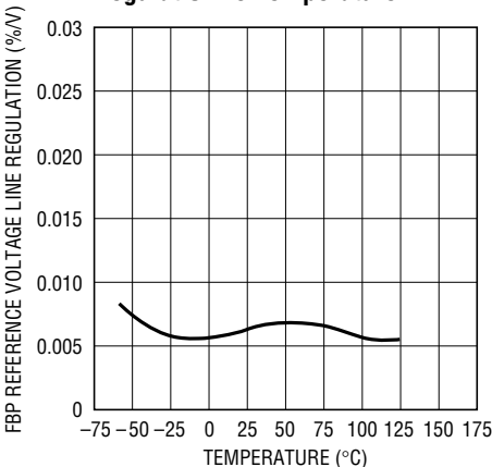
FBP Reference Voltage Line Regulation vs Temperature
