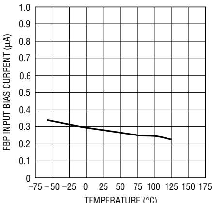
FBP Input Bias Current vs Temperature
