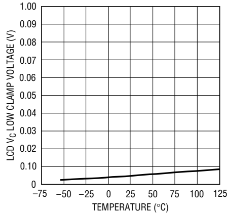
LCD V_C Low Clamp Voltage vs Temperature
