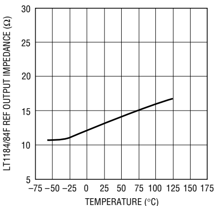
LT1184/84F REF Output Impedance vs Temperature
