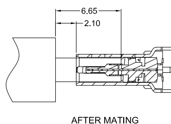
AFTER MATING
