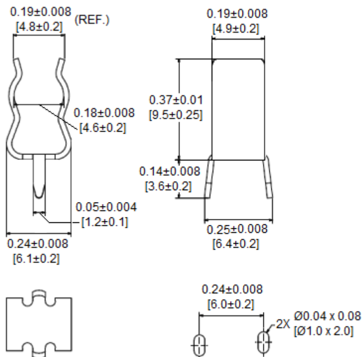
Recommended Mounting Holes
