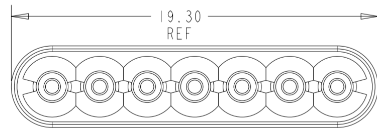
1-7 POSITION
