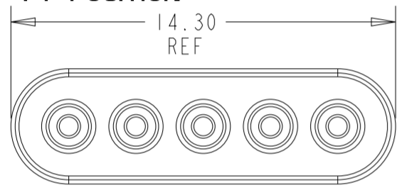
1-5 POSITION
