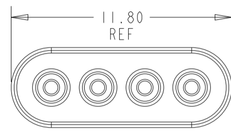
1-4 POSITION
