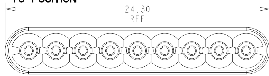
1-9 POSITION
