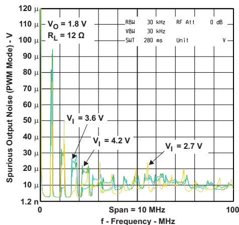
Figure 20. Spurious Output Noise (PWM Mode) vs Frequency
