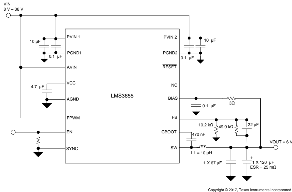
Figure 49. 6-V Output Power Supply
