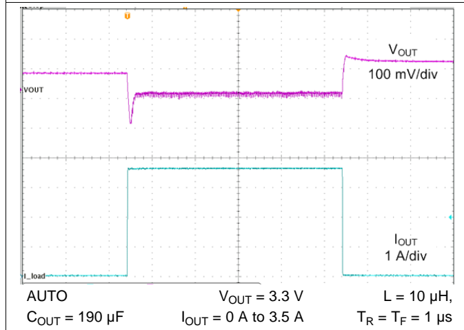
Figure 46. Load Transient
