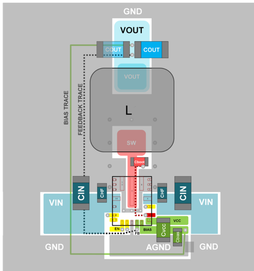
Figure 54. Recommended Layout for LMS36x5-Q1
