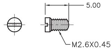
SCREW
