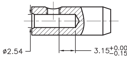
BODY
