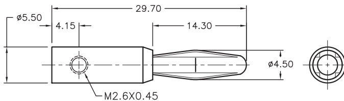
HANDLE
