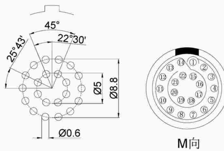
Pcb plate opening size (PCB板开孔尺寸)
