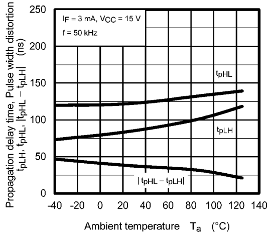
Fig. 12.2.20 t_{pHL} , t_{pLH} , |t_{pHL}-t_{pLH}| - T_a (Test Circuit Fig. 12.1.8)
