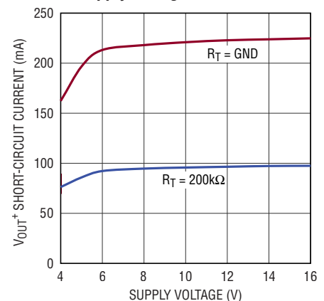
V_{OUT^+} Short-Circuit Current vs Supply Voltage
