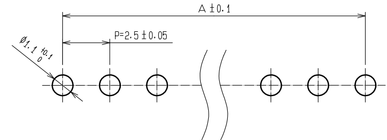
RECOMMENDED PATTERN(5:1)
