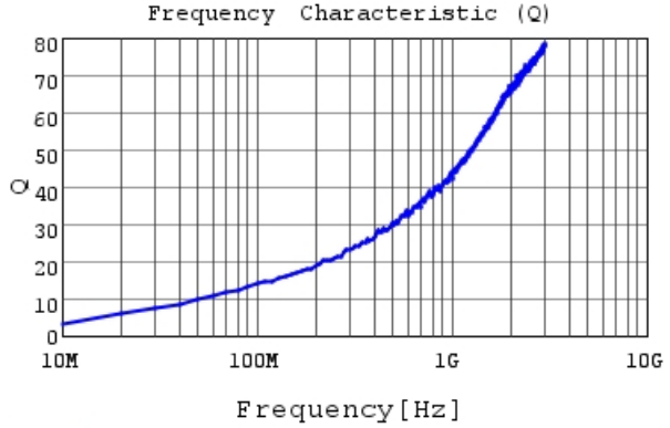
LQP03TN1N0C02 Q
