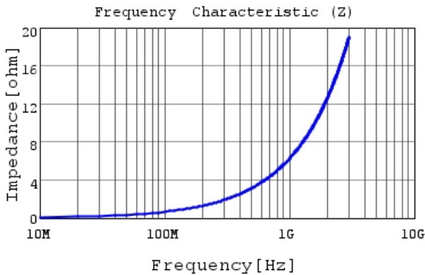
LQP03TN1N0C02 |Z|
