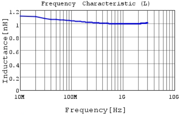
LQP03TN1N0C02 L
