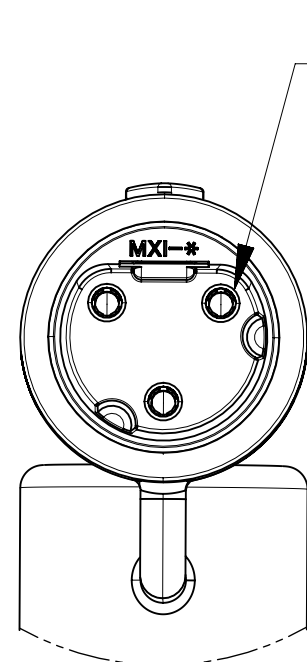
VIEW SHOWING KEYING OF 3 CIRCUIT VERSION
