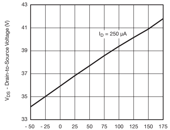
Drain Source Breakdown vs. Junction Temperature
