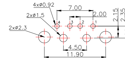
PCB.WELDING DRAWING (TOLERANCE:±0.05)
