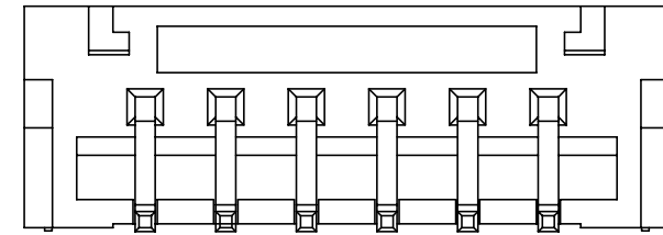
RECOMMENDER P.C.B LAYOUT TOP VIEW (GENERAY TOLERANCE ±0.10)
