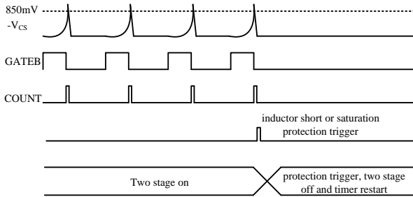
Fig.14 Inductor Short or Saturation Protection
