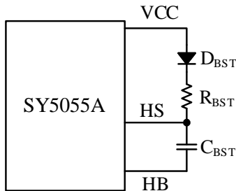
Fig.33 High Side Driver Power Supply Circuit
