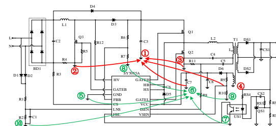
Fig. 36 Recommendation of Ground Connection
