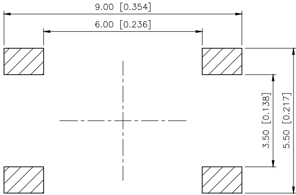
PCB LATOUT TOP VIEW
