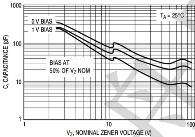
Typical Capacitance
