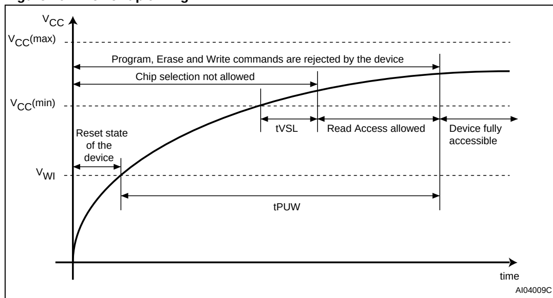
Figure 20. Power-up timing
