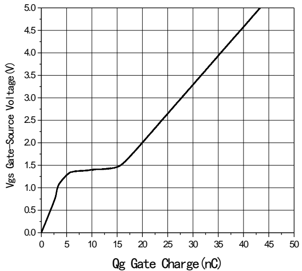
Fig6 Gate Charge
