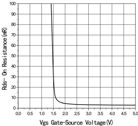
Fig5 R_{DS(on)} -Gate Drain voltage
