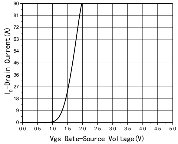
Fig2 Transfer Characteristics
