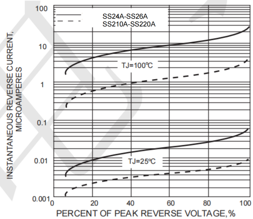
FIG. 4-TYPICAL REVERSE LEAKAGE CHARACTERISTICS
