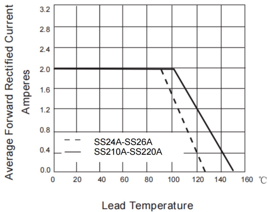
FIG. 1- DERATING CURVE OUTPUT RECTIFIED CURRENT
