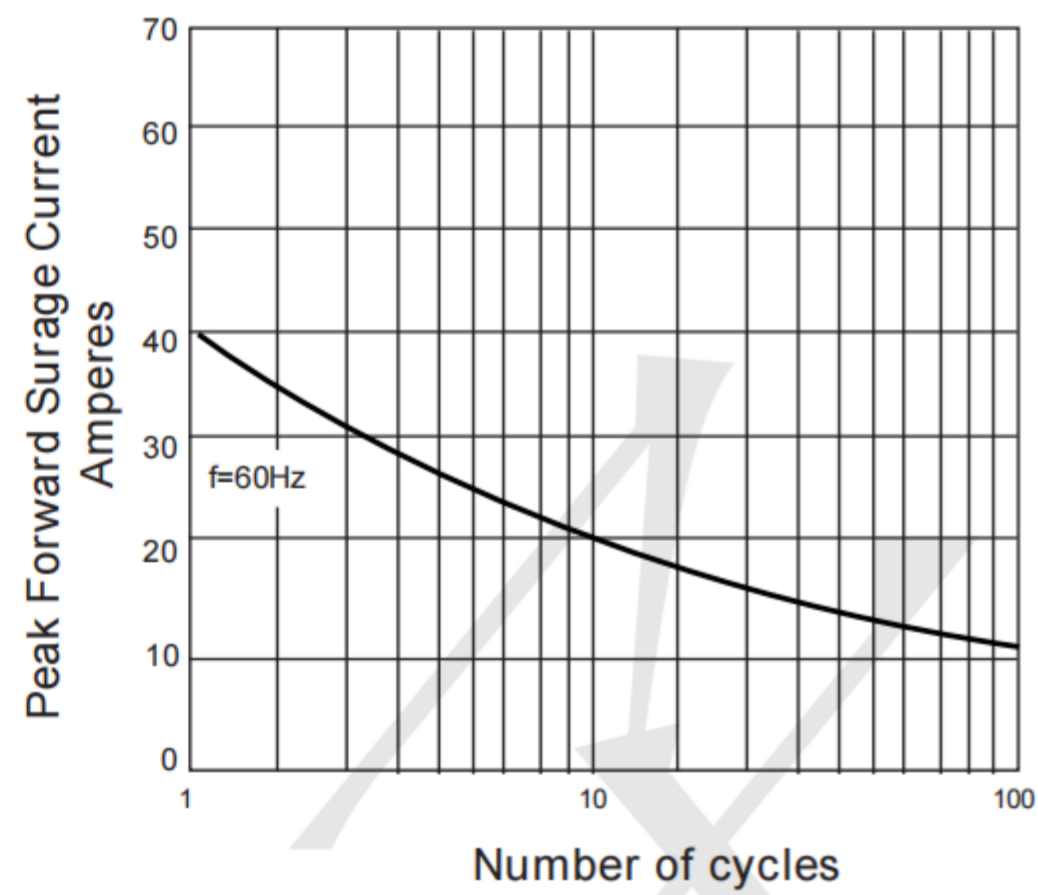
FIG. 2-MAXIMUM NON-REPETITIVE PEAK FORWARD SURGE CURRENT PER LEG
