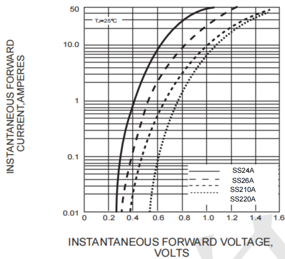
FIG. 3-TYPICAL FORWARD VOLTAGE CHARACTERISTICS
