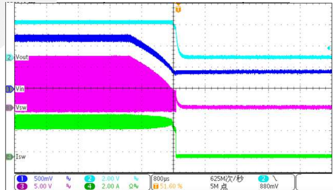
Shut down from VIN (VIN=12V, VOUT=3.3V, Load=1Ω)
