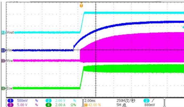
Start up from VIN (VIN=12V, VOUT=3.3V, Load=1Ω)
