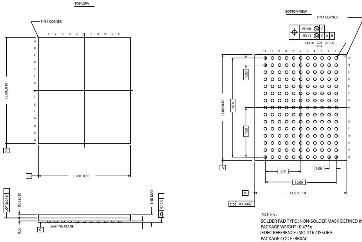
Figure 5. 165-Ball FBGA (13 x 15 x 1.4 mm)
