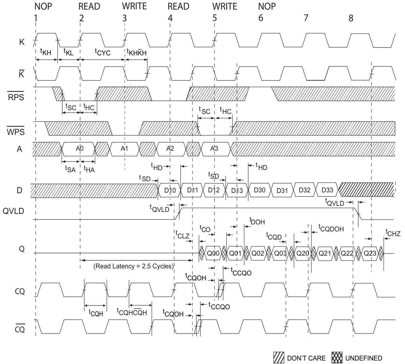
Figure 4. Waveform for 2.5 Cycle Read Latency
