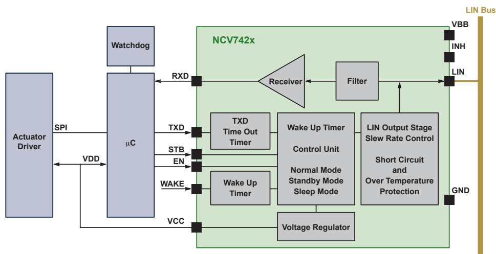
NCV742x LIN-SBC: LIN + LDO (5 or 3.3 V) up to 150 mA
