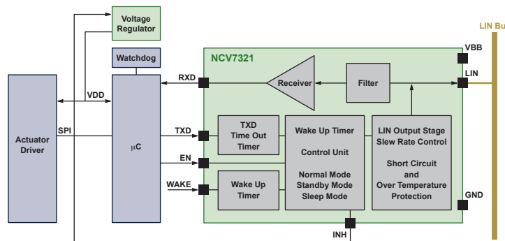
Standalone LIN Transceiver NCV7321
