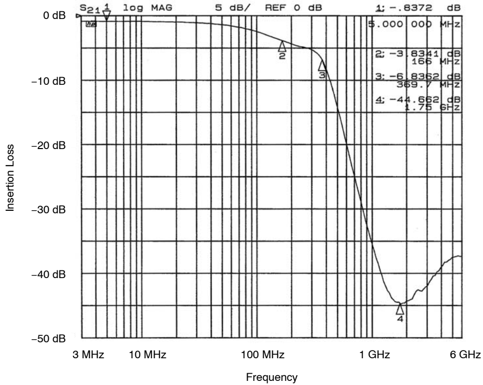
Figure 1. Filter 1 Insertion Loss (CM1460-04DE)
