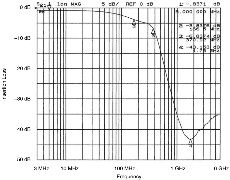
Figure 18. Filter 8 Insertion Loss (CM1460-08DE)
