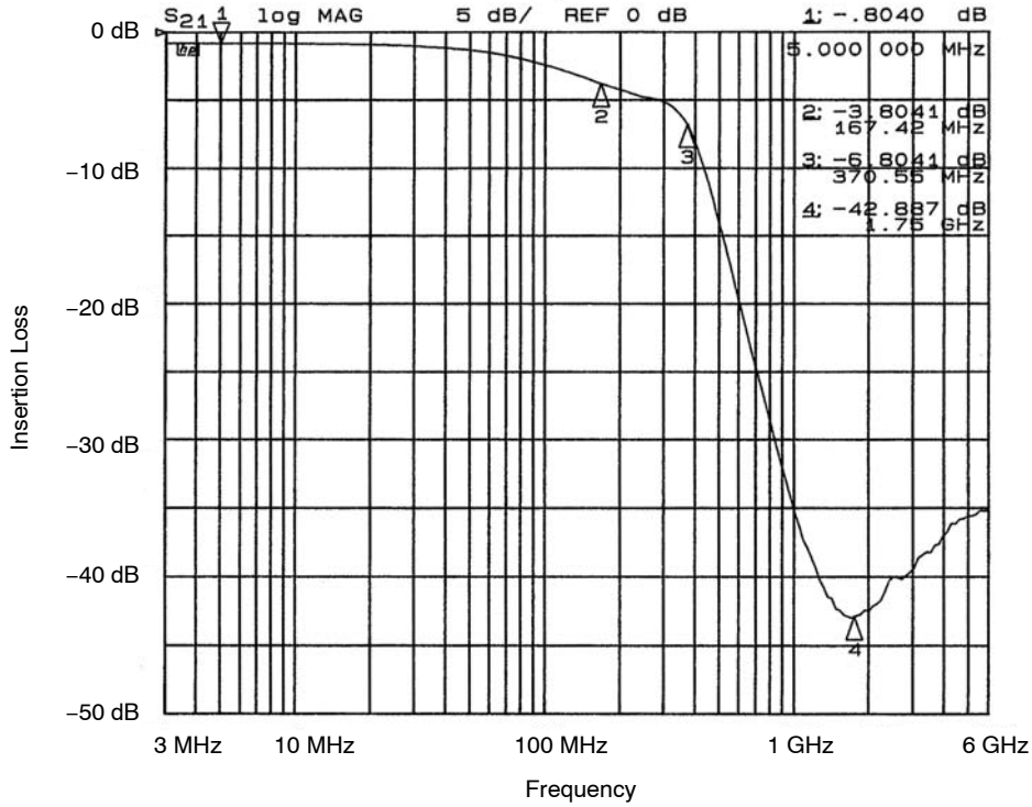
Figure 15. Filter 5 Insertion Loss (CM1460-08DE)
