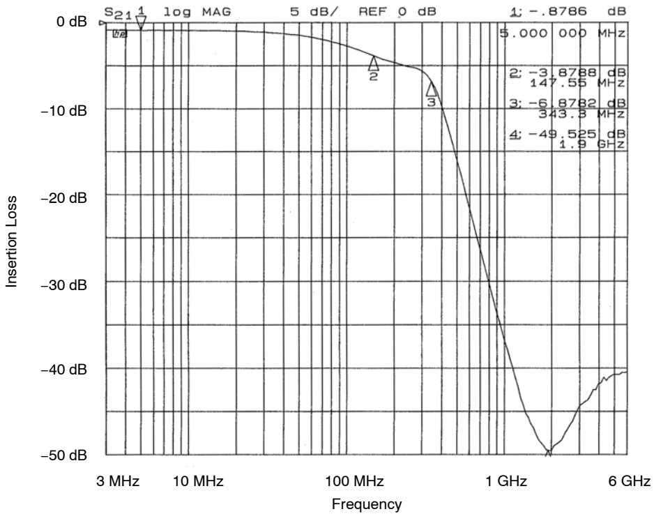
Figure 8. Filter 4 Insertion Loss (CM1460-06DE)
