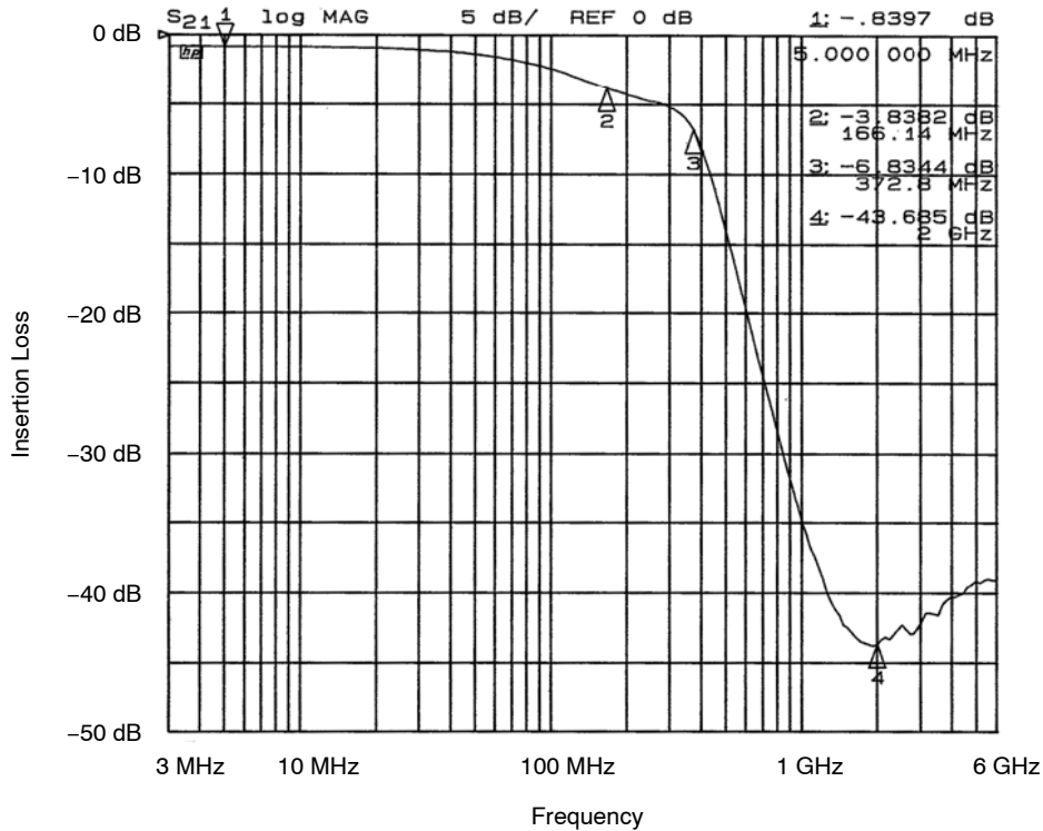
Figure 2. Filter 2 Insertion Loss (CM1460-04DE)
