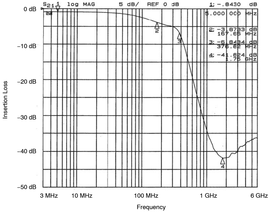
Figure 13. Filter 3 Insertion Loss (CM1460-08DE)
