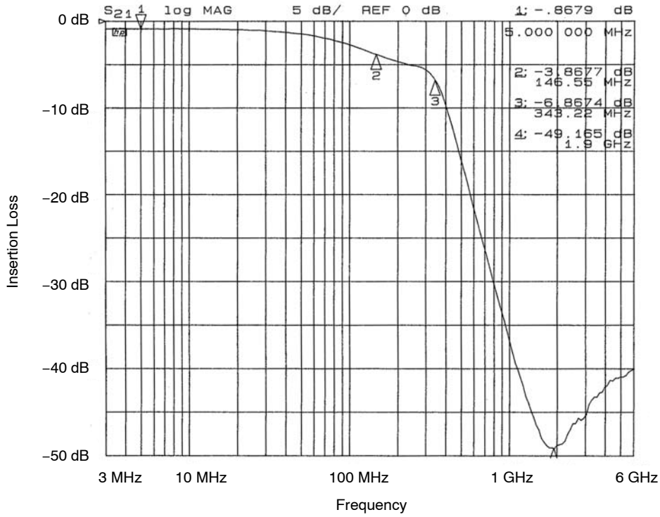
Figure 7. Filter 3 Insertion Loss (CM1460-06DE)
