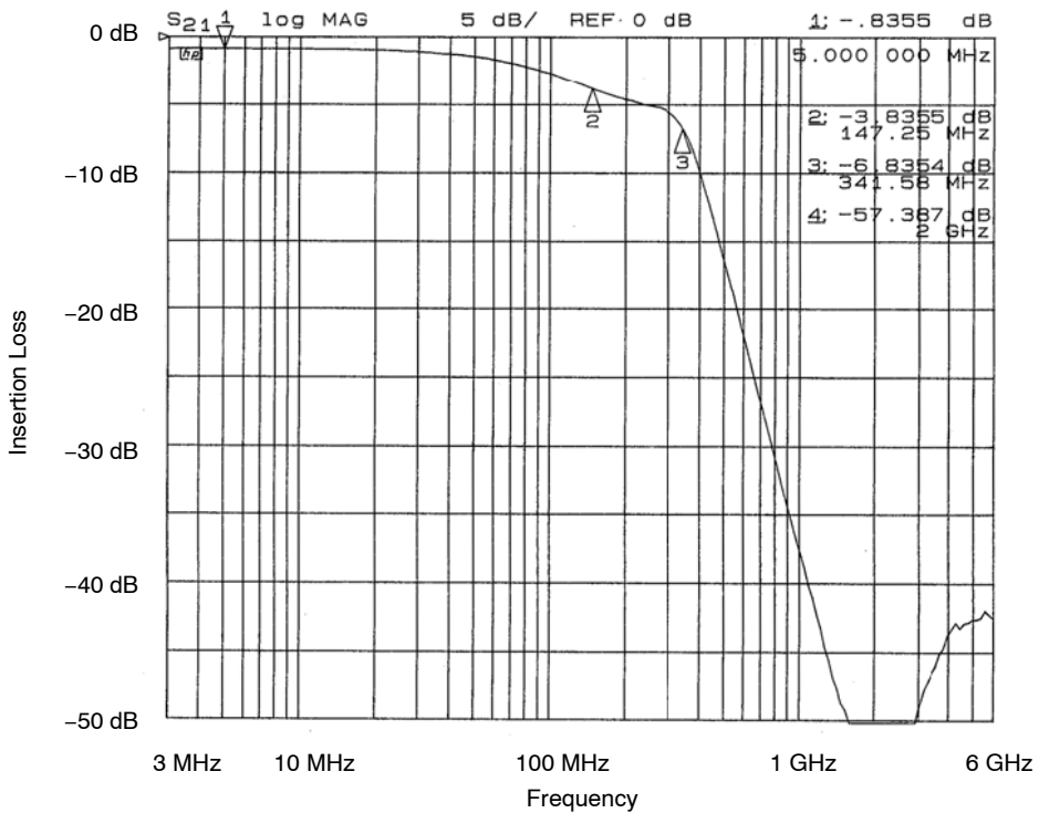
Figure 10. Filter 6 Insertion Loss (CM1460-06DE)
