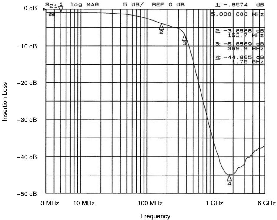
Figure 4. Filter 4 Insertion Loss (CM1460-04DE)
