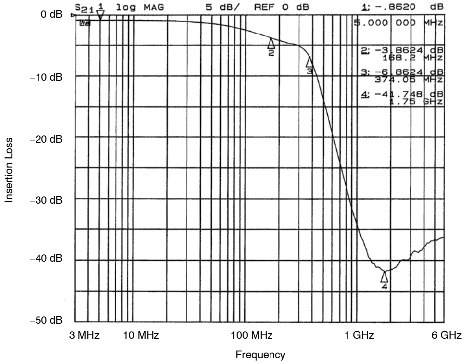
Figure 17. Filter 7 Insertion Loss (CM1460-08DE)
