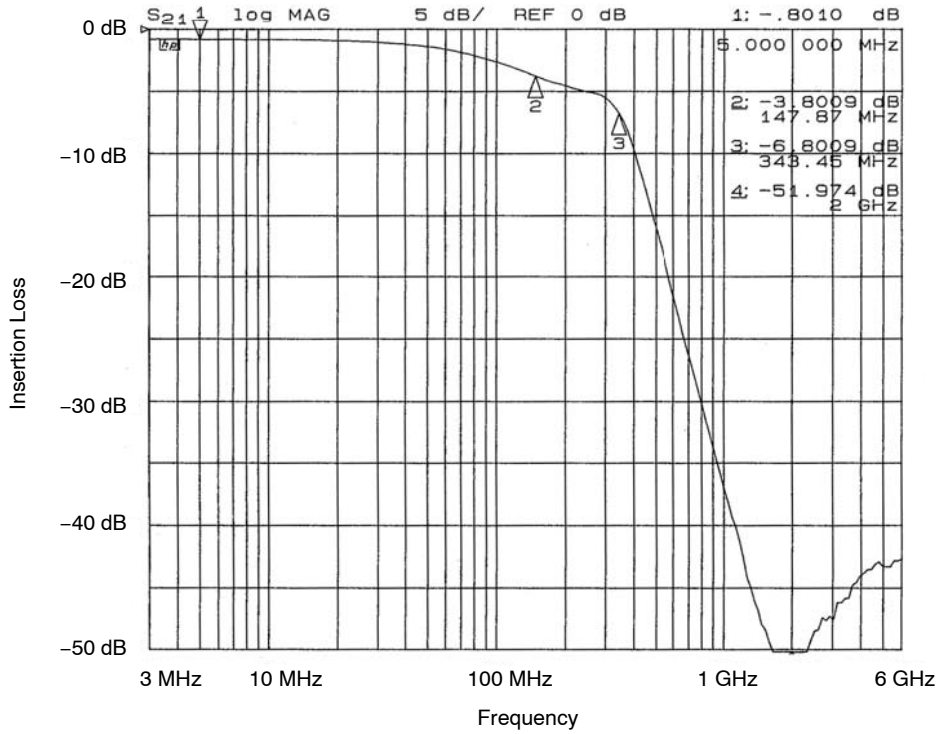
Figure 9. Filter 5 Insertion Loss (CM1460-06DE)
