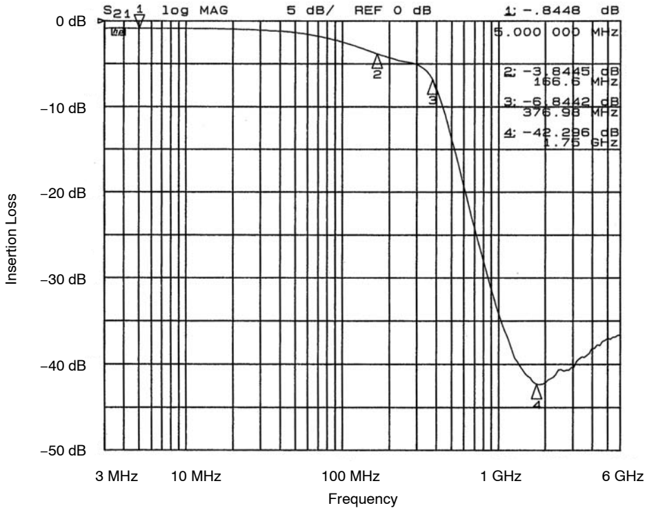
Figure 12. Filter 2 Insertion Loss (CM1460-08DE)
