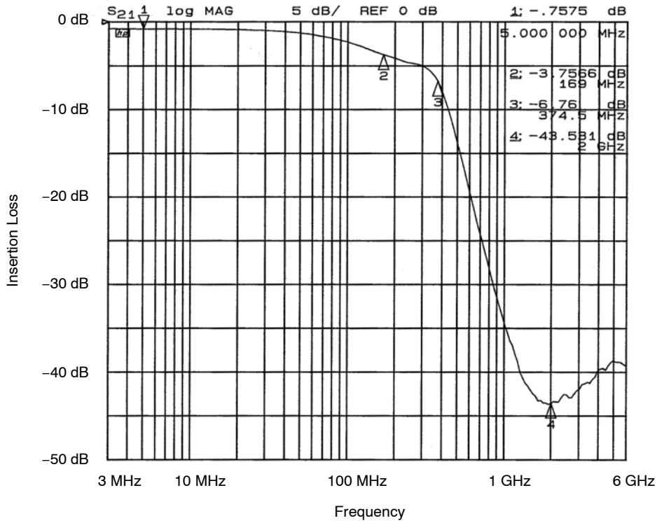
Figure 3. Filter 3 Insertion Loss (CM1460-04DE)
