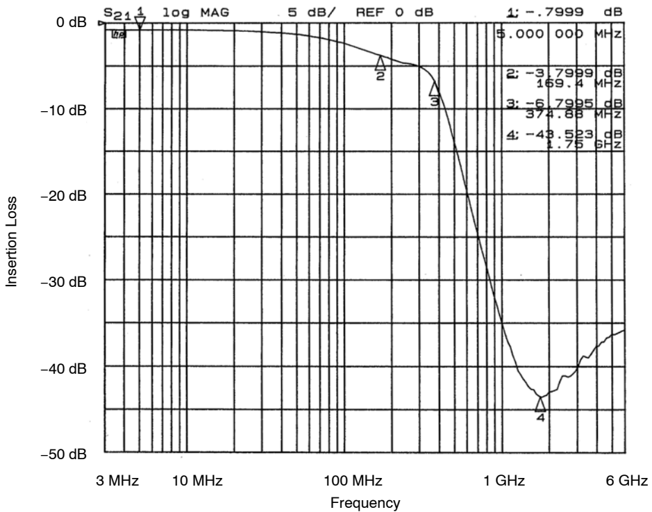
Figure 14. Filter 4 Insertion Loss (CM1460-08DE)
