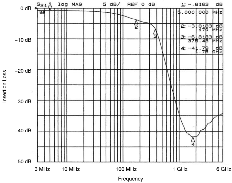
Figure 11. Filter 1 Insertion Loss (CM1460-08DE)
