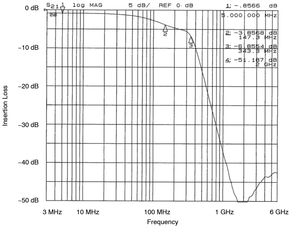
Figure 6. Filter 2 Insertion Loss (CM1460-06DE)
