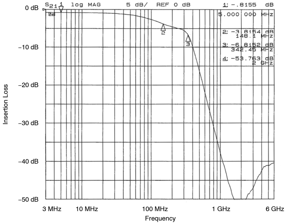
Figure 5. Filter 1 Insertion Loss (CM1460-06DE)
