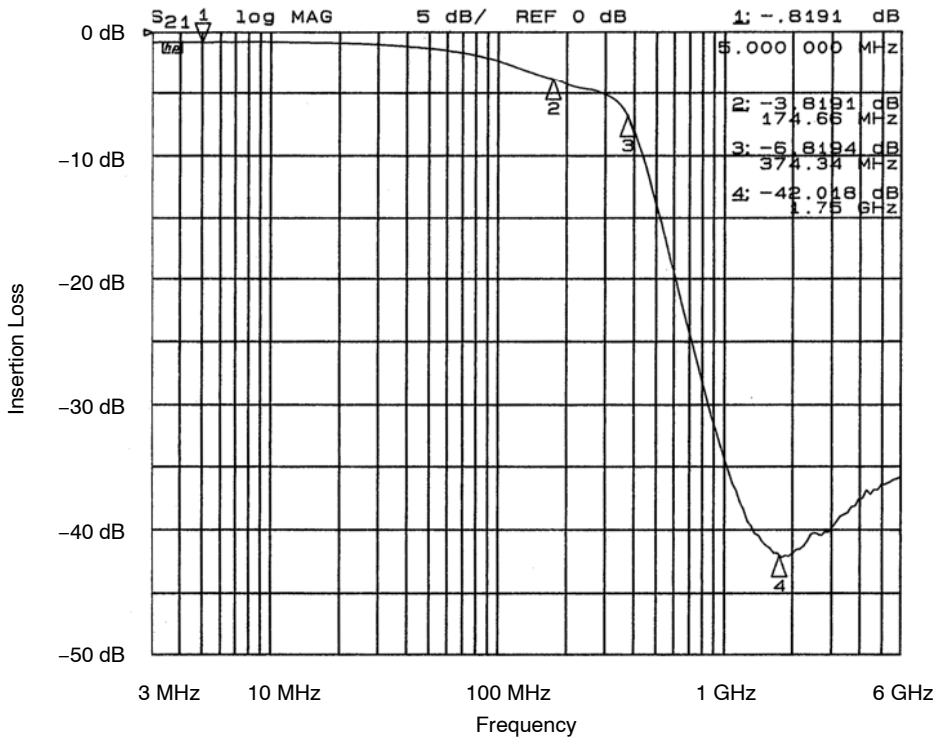
Figure 16. Filter 6 Insertion Loss (CM1460-08DE)
