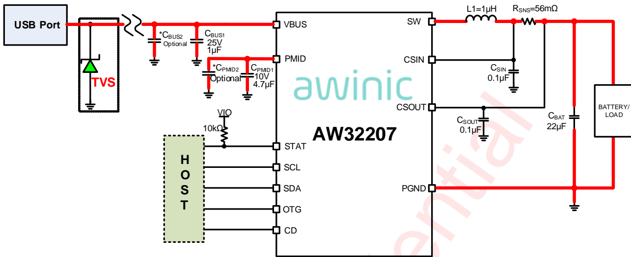
Figure 4 AW32207 Application Circuit
