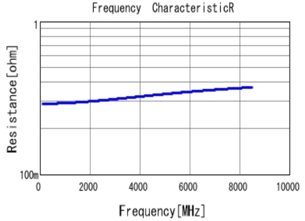
GJM0335C1E1R2BB01 R DC0V, 25degC
