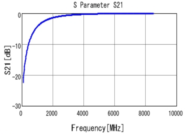
■ GJM0335C1E1R2BB01 S21 DCOV, 25degC
