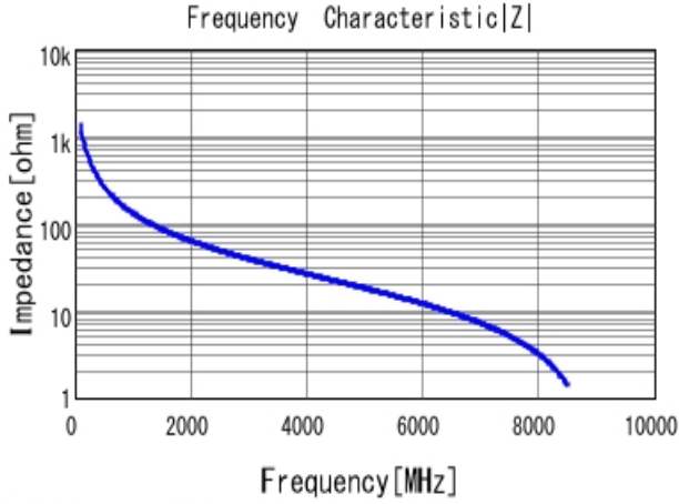
GJM0335C1E1R2BB01 |Z| DC0V, 25degC
