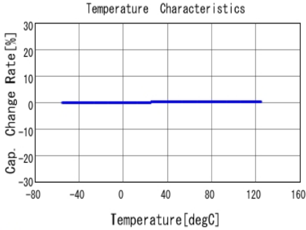
■ GJM0335C1E1R2BB01 C-Temp. capchange, DCOV, AC1Vrms
