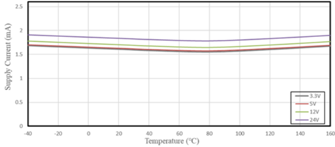
Supply current VS. Temperature
