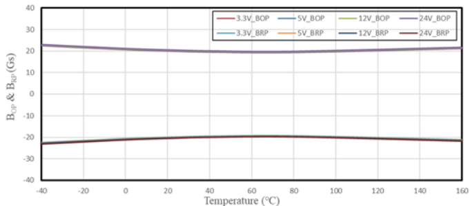
SC2442 B OP & B RP VS. Temperature
