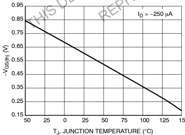
Figure 11. Threshold Voltage
