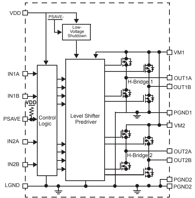
Figure 2. 17C724 Simplified Internal Block Diagram
