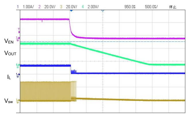
(18) Enable Shutdown (VIN=30.0V,VOUT=3.3V,IOUT=0.6A)
