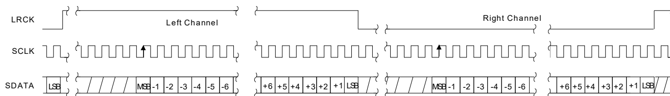
Figure 6. Format 2, Right Justified 16-Bit Data Format 3, Right Justified 24-Bit Data Format 4, Right Justified 20-Bit Data. (Available in Control Port Mode only)
