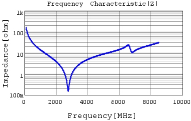
GJM1555C1H100JB01 |Z| DCOV, 25degC
