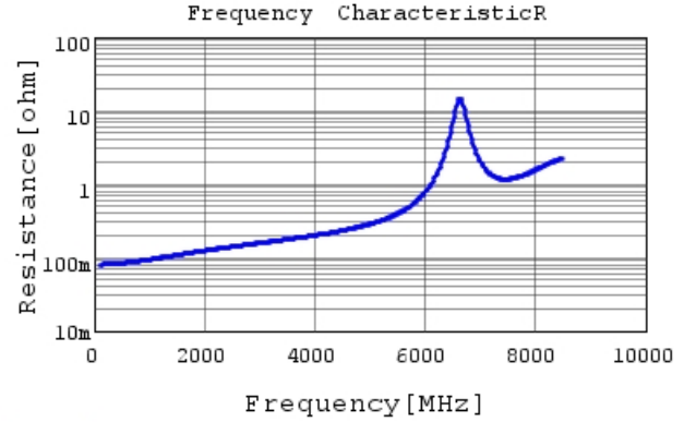
GJM1555C1H100JB01 R DCOV, 25degC
