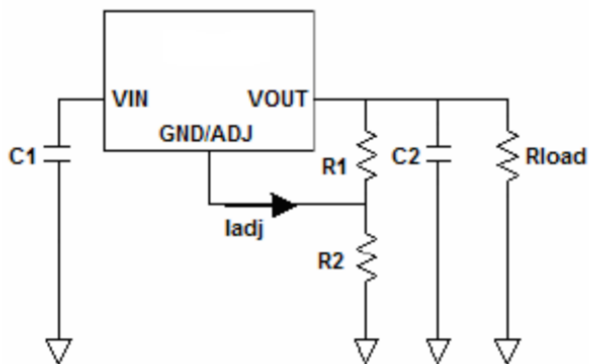
AMS1117 adjustable output voltage
