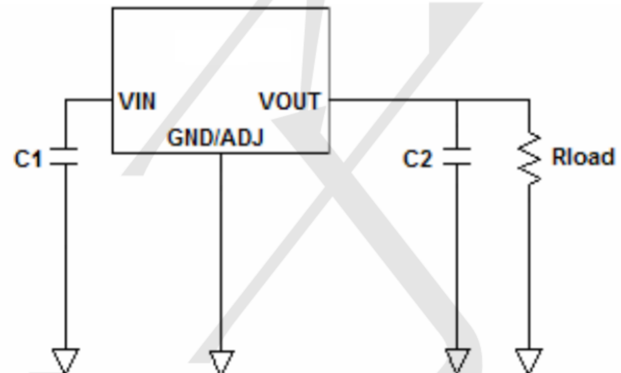
AMS1117 fixed output
