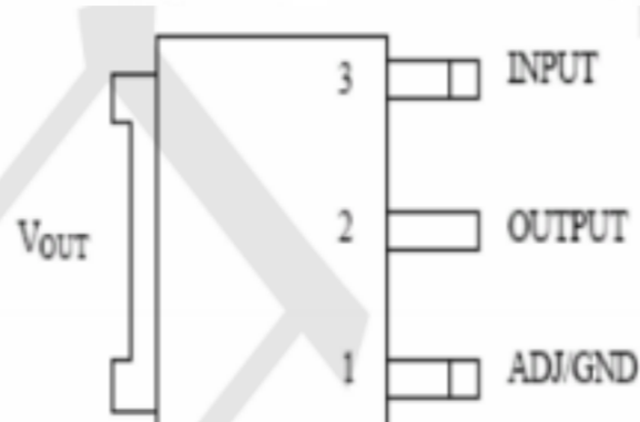
TO-252
