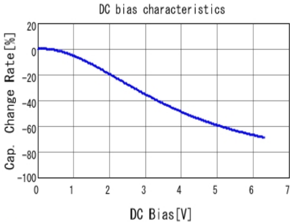
■ GRM188D70J106MA73 C-DC bias capchange, 25.0degC, AC1V
