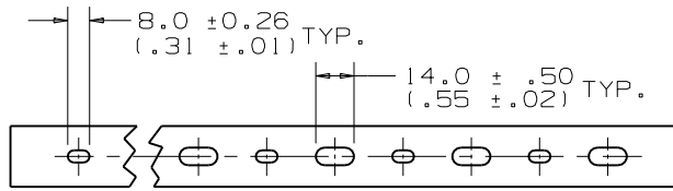
FOR 25mm, 37.5mm, 50mm, WIDTH DUCT
