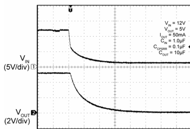
Fast Turn-Off
