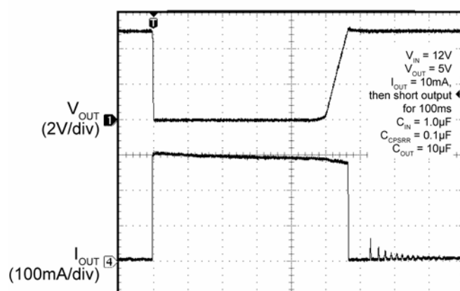
Current Limit
