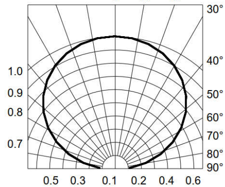
Fig.6-Radiation Diagram Ta=25°C
