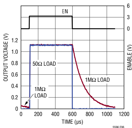
Figure 6. Output Voltage Turn-Off Transient for 1MΩ||11pF and 50Ω Load Impedance. Input Power 0dBm, Input Frequency 2140MHz.
