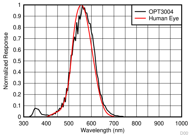
Figure 7-2. Spectral Response vs Wavelength
