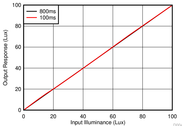
Figure 7-6. Output Response vs Input Illuminance (Mid Range = 0 lux to 100 lux)
