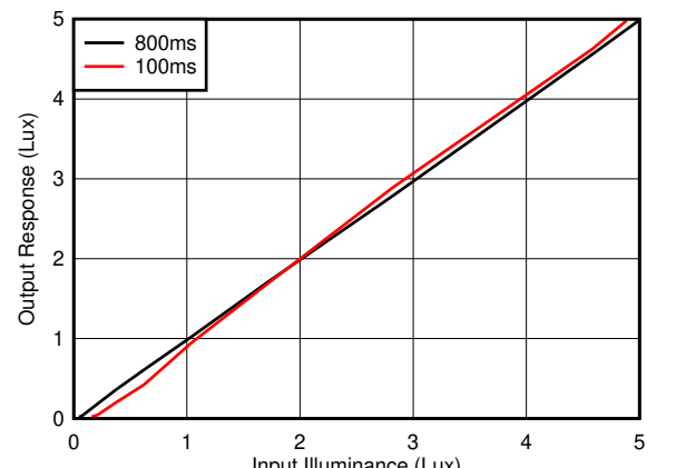
Figure 7-7. Output Response vs Input Illuminance (Low Range = 0 lux to 5 lux)
