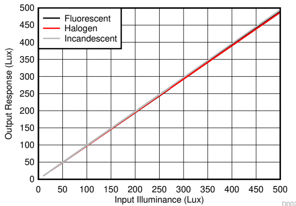
Figure 7-4. Output Response vs Input Illuminance, Multiple Light Sources (Fluorescent, Halogen, Incandescent)
