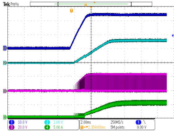
Figure 19. Power up
