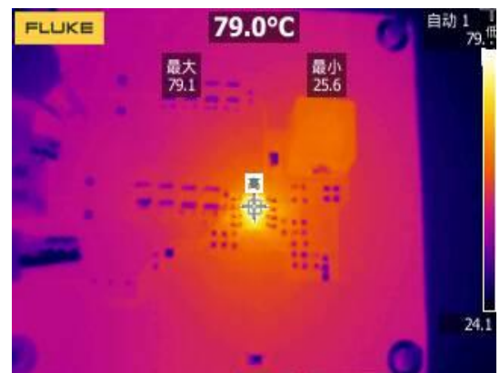
Figure 24. Thermal, 3.3Vout/5A
