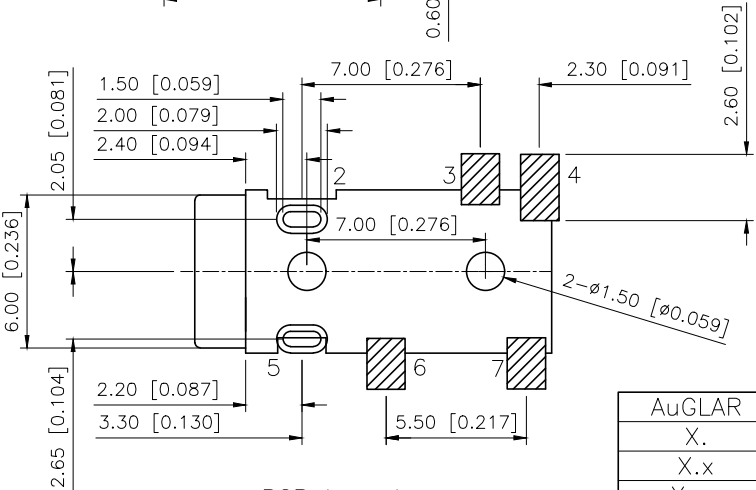
PCB Layout
