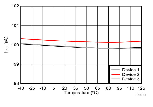
Figure 6-28. Reference Current vs Temperature
