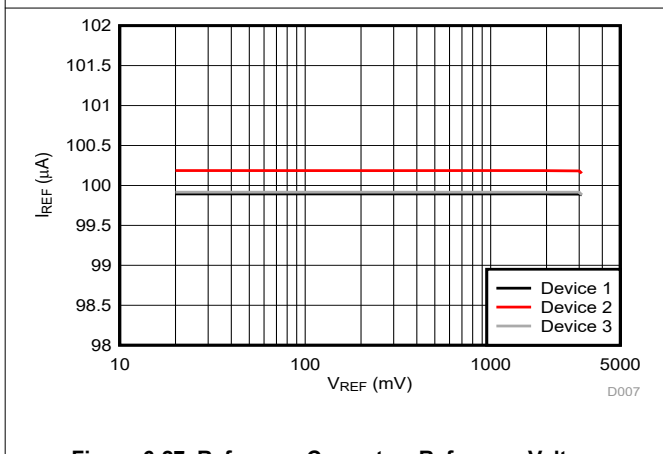
Figure 6-27. Reference Current vs Reference Voltage
