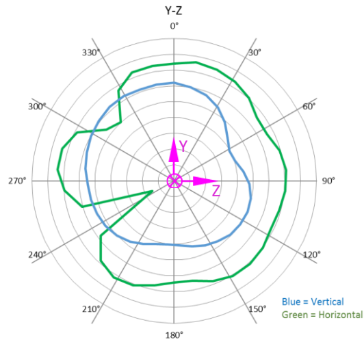
Figure 18 – Y-Z Plane Antenna Pattern
