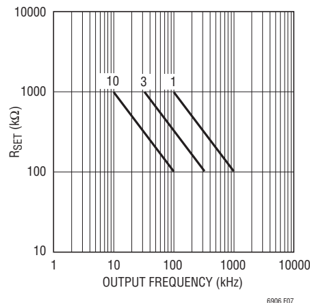
Figure 7. R_{SET} vs Desired Output Frequency (LTC6906)
