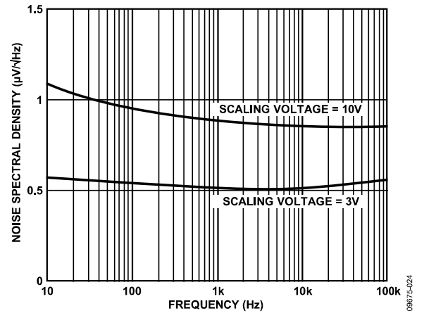
Figure 11. Noise Spectral Density vs. Frequency
