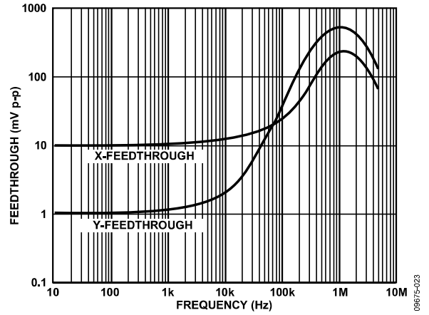
Figure 10. AC Feedthrough vs. Frequency
