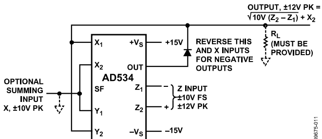
Figure 19. Square-Rooter Connection
