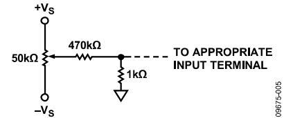
Figure 3. Optional Trimming Configuration
