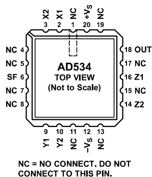
Figure 6. LCC (E-20-1) Pin Configuration
